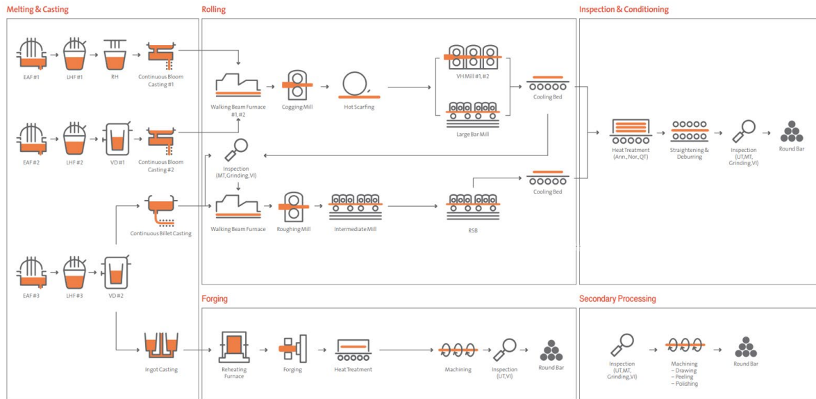
Figure 1 Manufacturing Process
